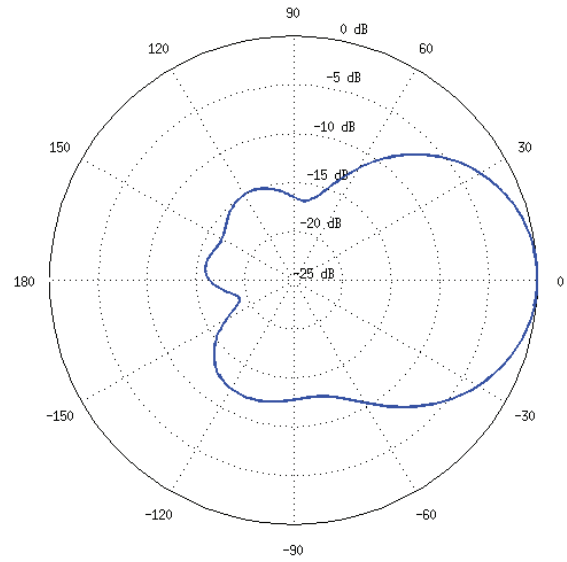
Horizontal Elevation
