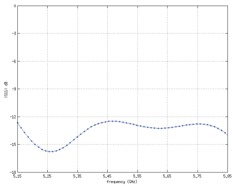
Return Loss
