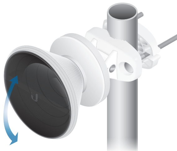
Pole-Mounting Using the U-OMT-MOUNT
