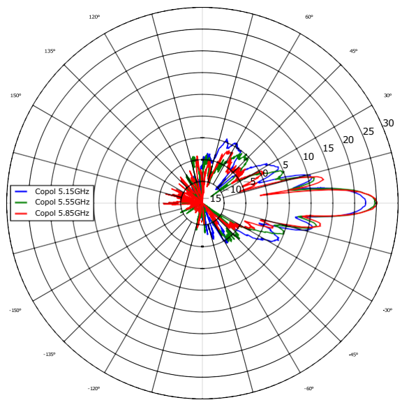
Elevation, Vertical
