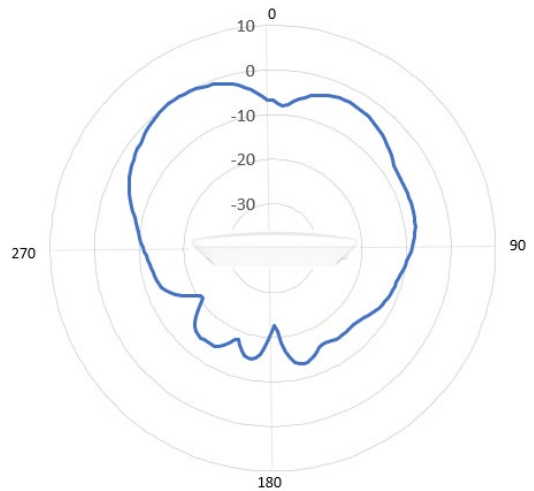
IoT Antenna Normalized Elevation Gain [dB]
