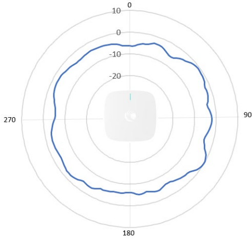
6 GHz Antenna Normalized Azimuth Gain [dB]
