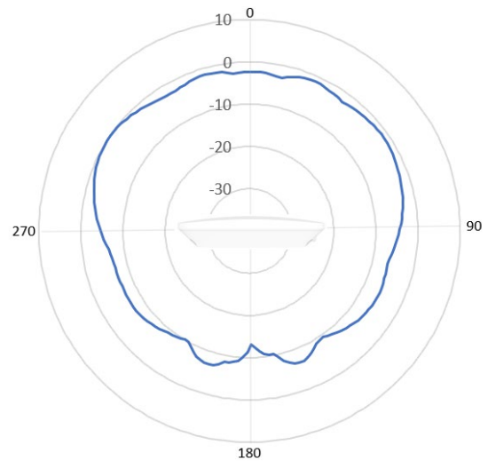
2 GHz Antenna Normalized Elevation Gain [dB]
